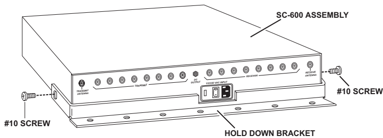
Figure 8 SC-600 Hold Down Bracket Rear View
