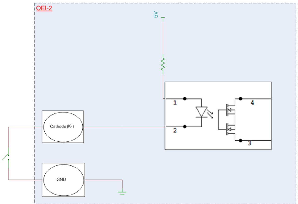
FIGURE 2. GPIO Input Diagram
