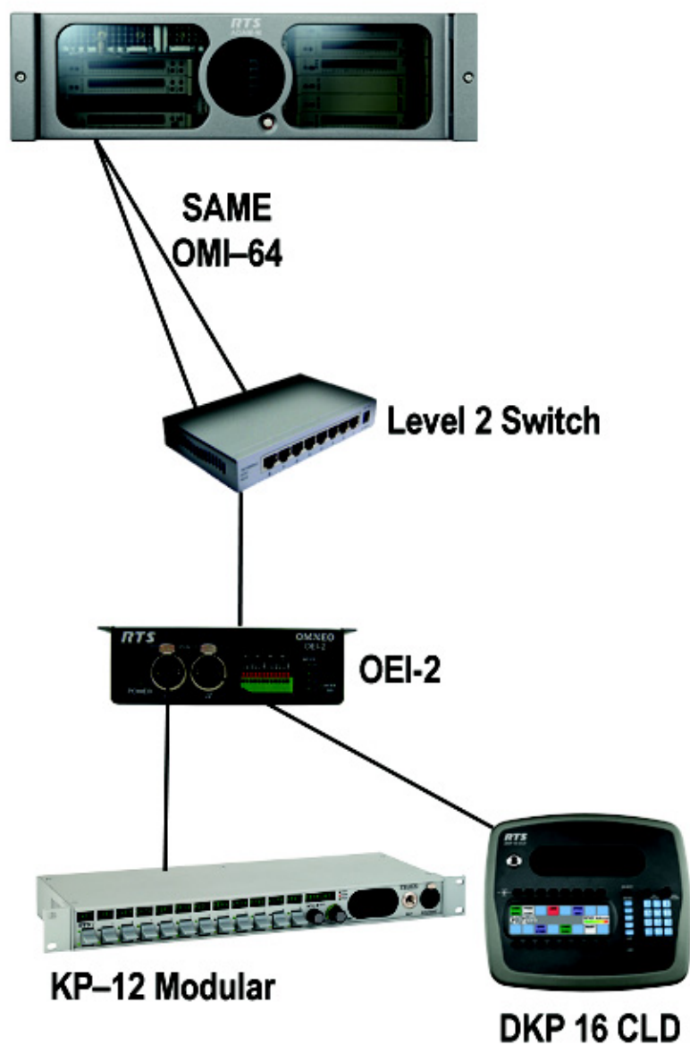
FIGURE 3. Same Frame, Same OMI Card System
