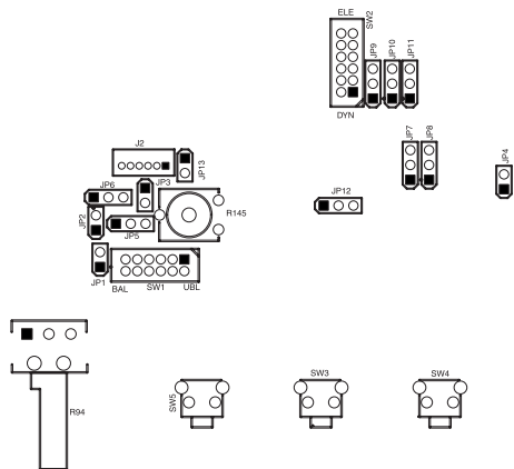
Figure 4. Board Number 9 0 30-7740-000.
