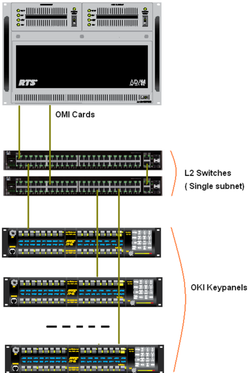
FIGURE 3. OMNEO Single Subnet System
