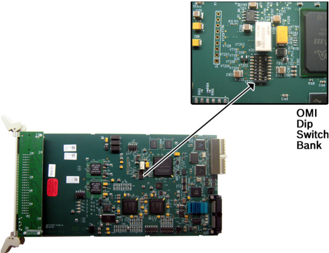
FIGURE 2. OMI DIP Switch Bank
