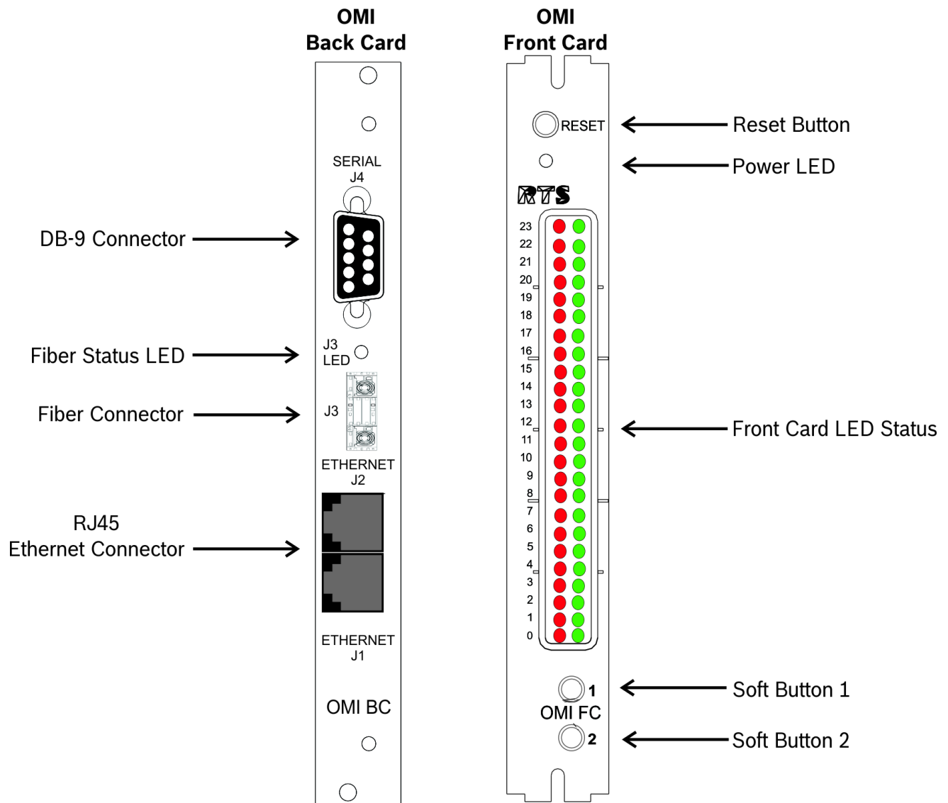
FIGURE 1. OMI Reference View
