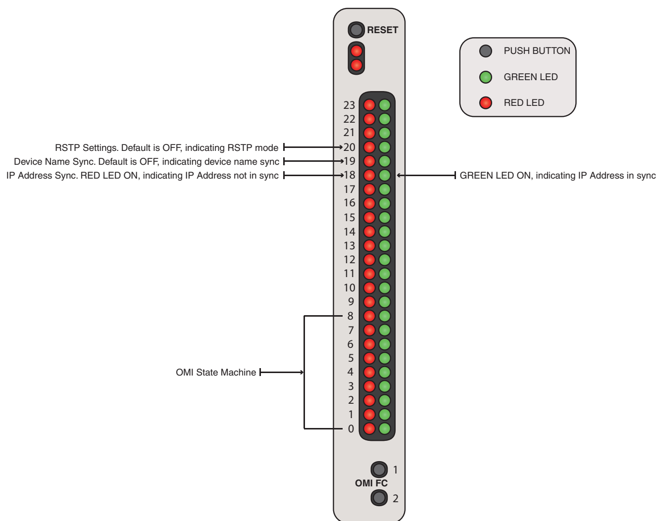
FIGURE 24. OMI–Page 0 LED Indicators
